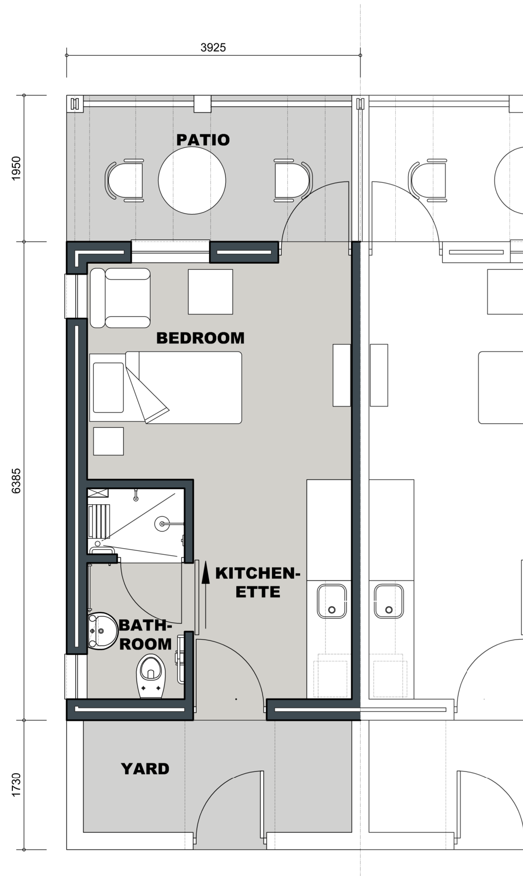
TYPE 1: ASSISTED LIVING UNIT scale 1:50 Proposed Lifestyle Village for Ellenrust Properties CC, Stilbaai.
